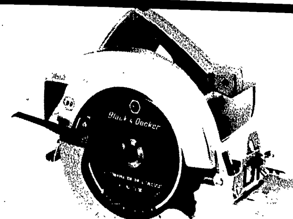
BLACK & DECKER 7-1/4" CIRCULAR SAW 1.5 HP. Double Insulated, Sawdust Ejection Chute Cutting Depth: 90° 2-7/16"; 45° 1-7/8"
